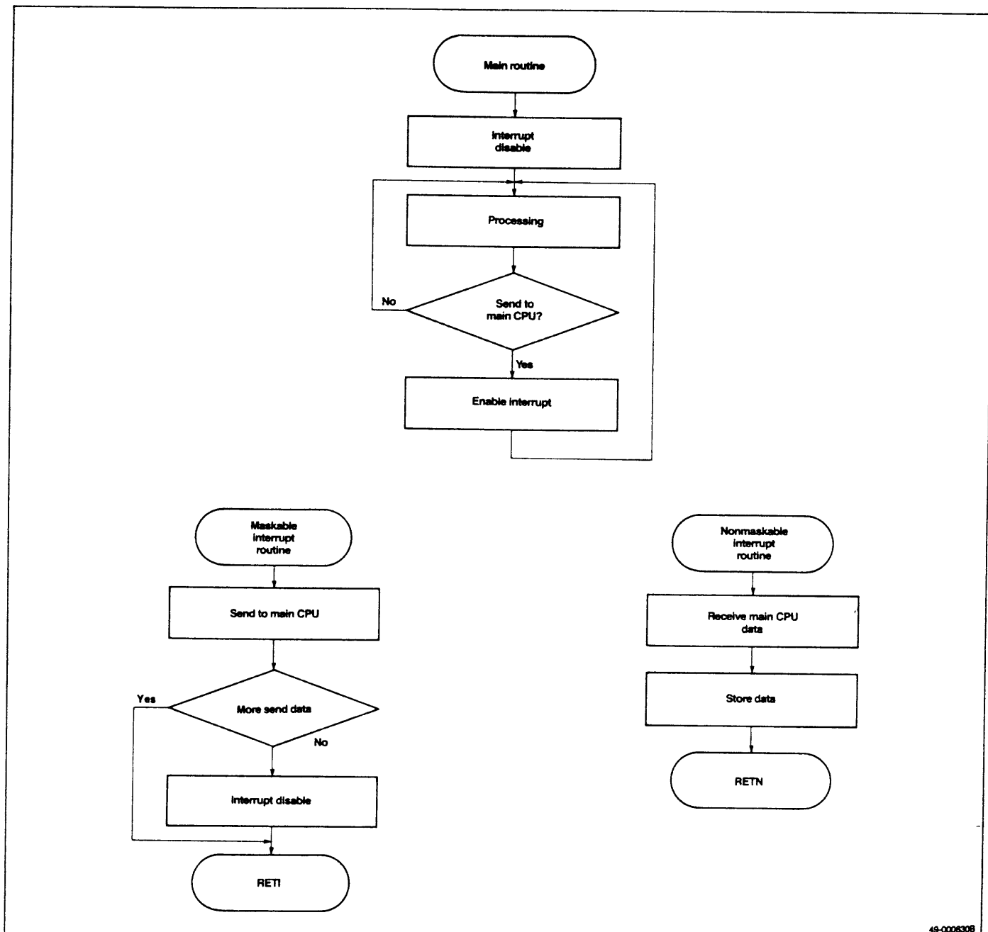
Figure 19. Sub CPU Flowchart
